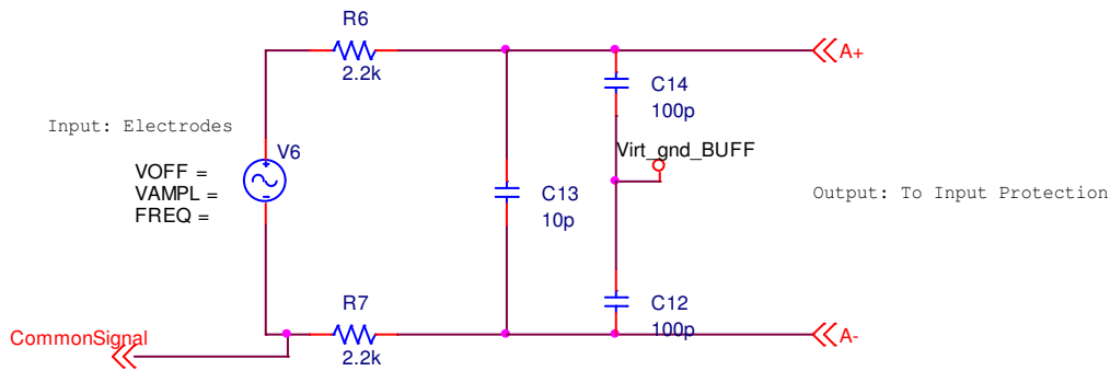
Figure 2: High Frequency Noise Rejection Circuit
