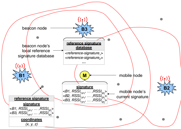
Figure 8: The MoteTrack location system. B1, B2, and B3 are beacon nodes, which broadcast beacon messages at various frequencies and transmission powers ( f_{1p_1}, \dots, f_{ip_j} ). Each beacon node stores a subset of all reference signatures. M is a mobile node that can hear from all three beacon nodes. It aggregates beacon messages received over some time period into a signature. The areas enclosed by perimeter lines indicate the reachability of beacon messages from the corresponding beacon node. The dots denote the known locations where reference signatures were collected.
