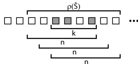
Figure 5: In this example, if the adversary holds a set \hat{S} of k = 3 shares (shown as shaded boxes), then we define p(\hat{S}) as the union of all (three) windows of n = 6 shares containing the original k shares. We require that the adversary be unable to recover keys for periods outside of p(\hat{S}) . The figure assumes \lambda = 0 . If \lambda = 1 , then p(\hat{S}) would include two additional shares: one before and one after the set p(\hat{S}) currently shown.
