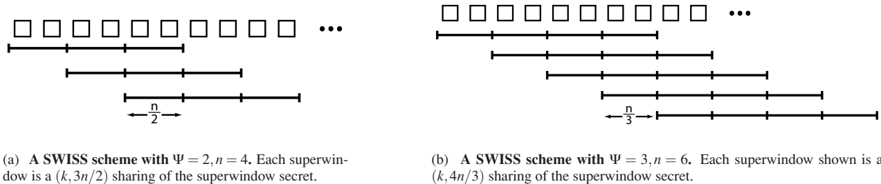
Figure 7: Additional SWISS examples We can create additional SWISS schemes by increasing the number of windows per superwindow while decreasing the number of shares in each window. As we increase the number of windows, \lambda decreases, but the number of shares that must be held in each time period increases.
